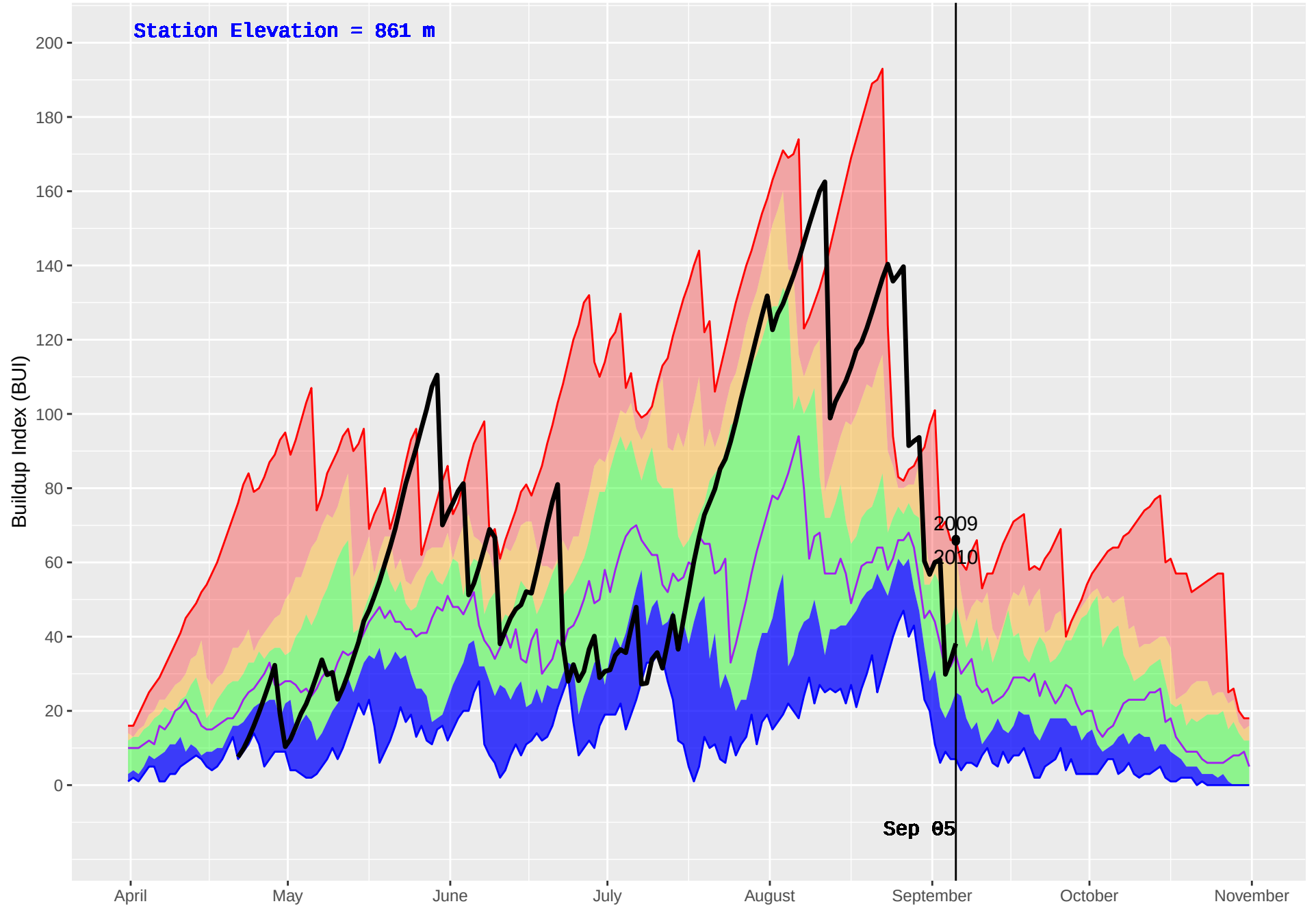
BLAEBERRY (866) : Historical (2004–2016) and Current (2018) Daily Buildup Index (BUI)
