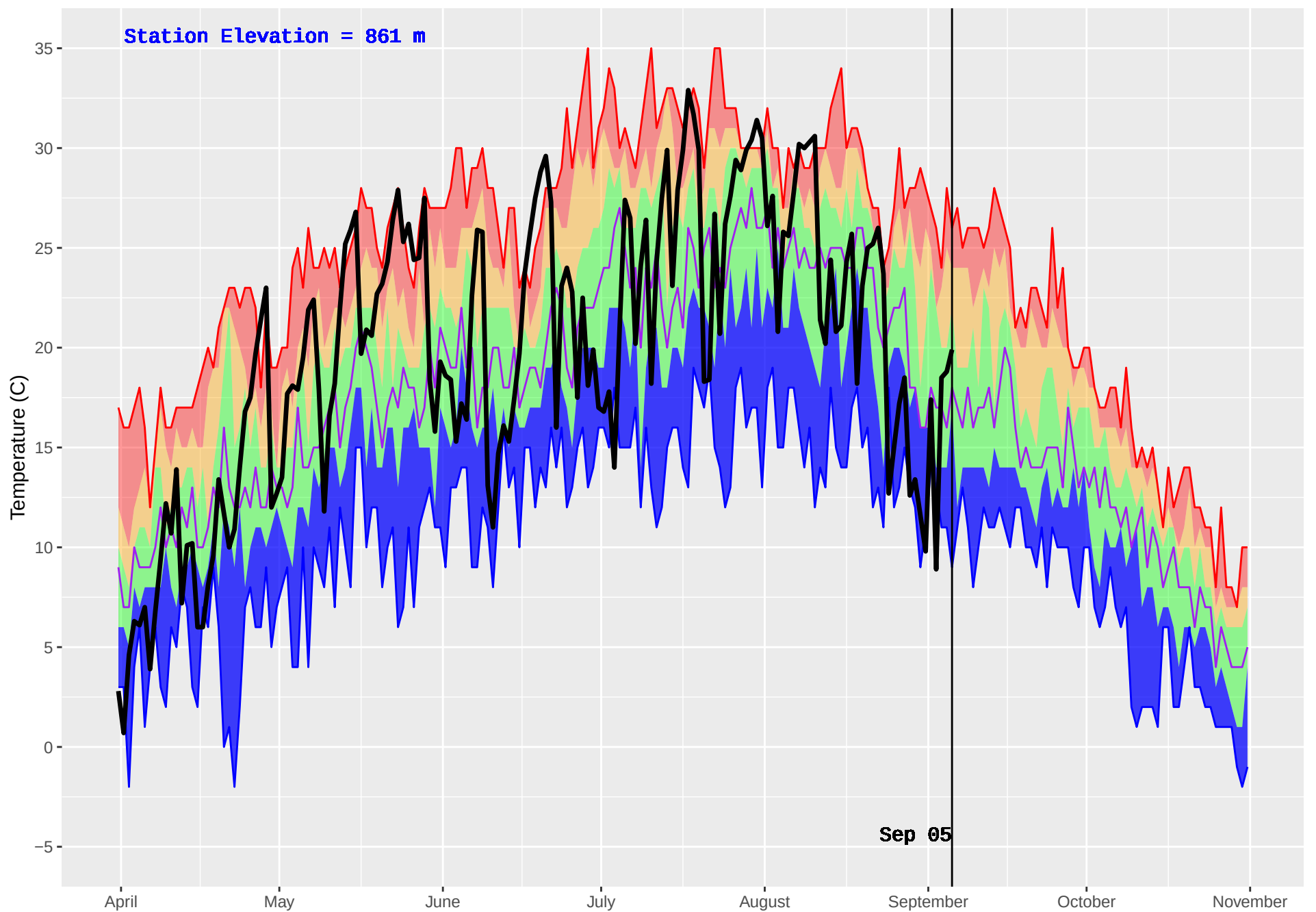
BLAEBERRY (866) : Historical (2004–2016) and Current (2018) Daily Temperature
