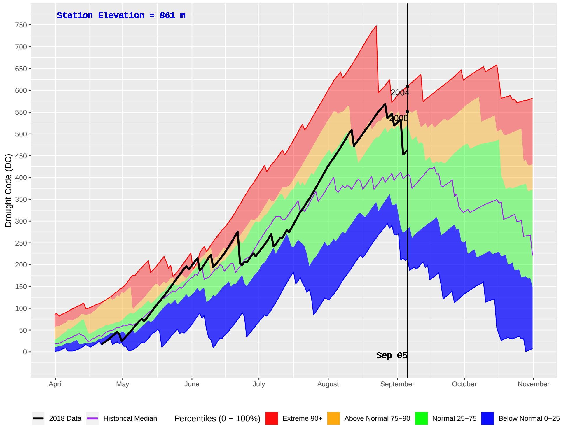
BLAEBERRY (866) : Historical (2004–2016) and Current (2018) Daily Drought Code (DC)
