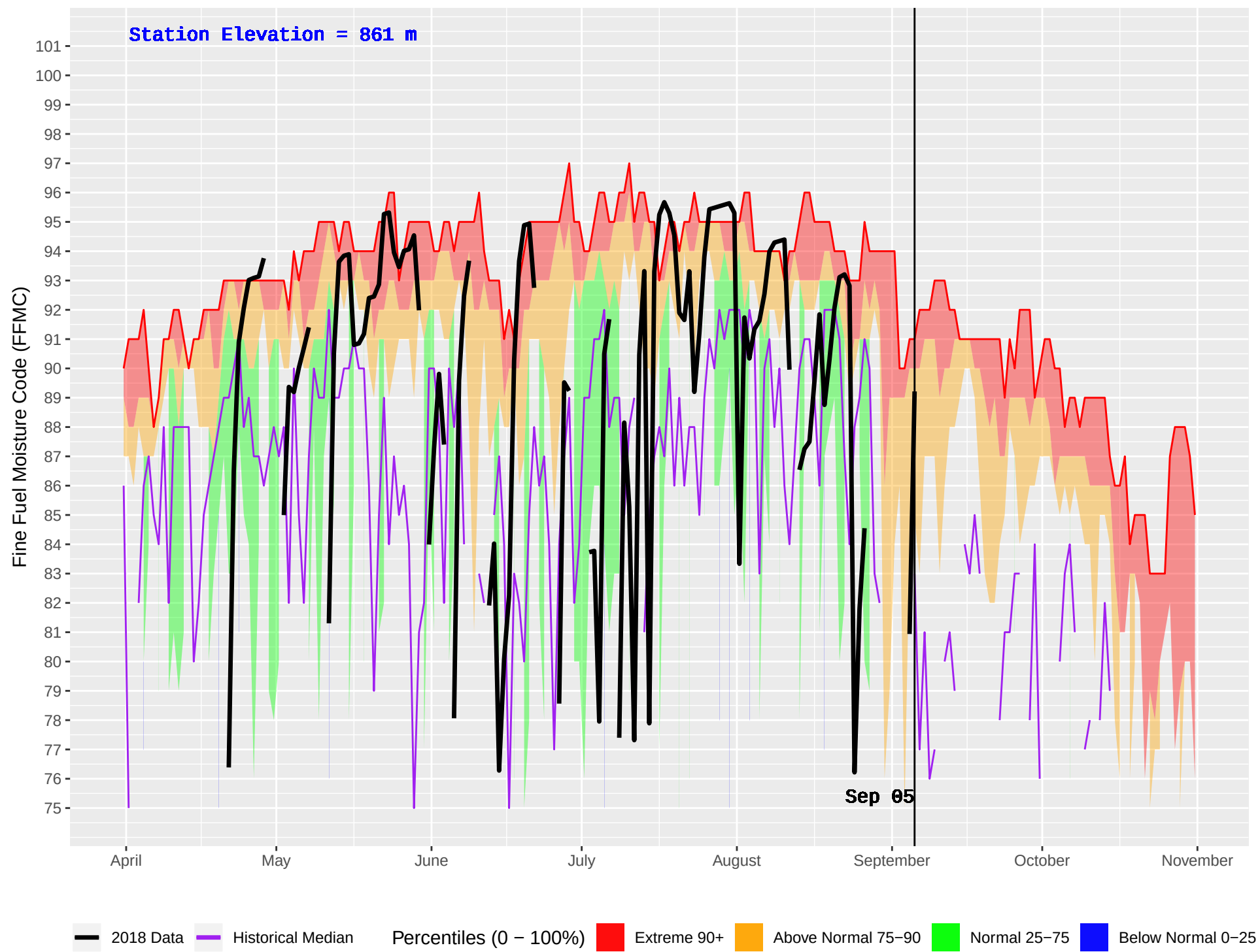
BLAEBERRY (866) : Historical (2004–2016) and Current (2018) Daily Fine Fuel Moisture Code (FFMC)
