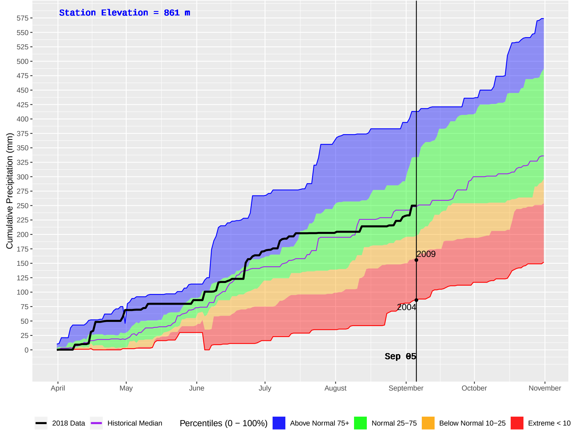
BLAEBERRY (866) : Historical (2004–2016) and Current (2018) Daily Cumulative Precipitation
