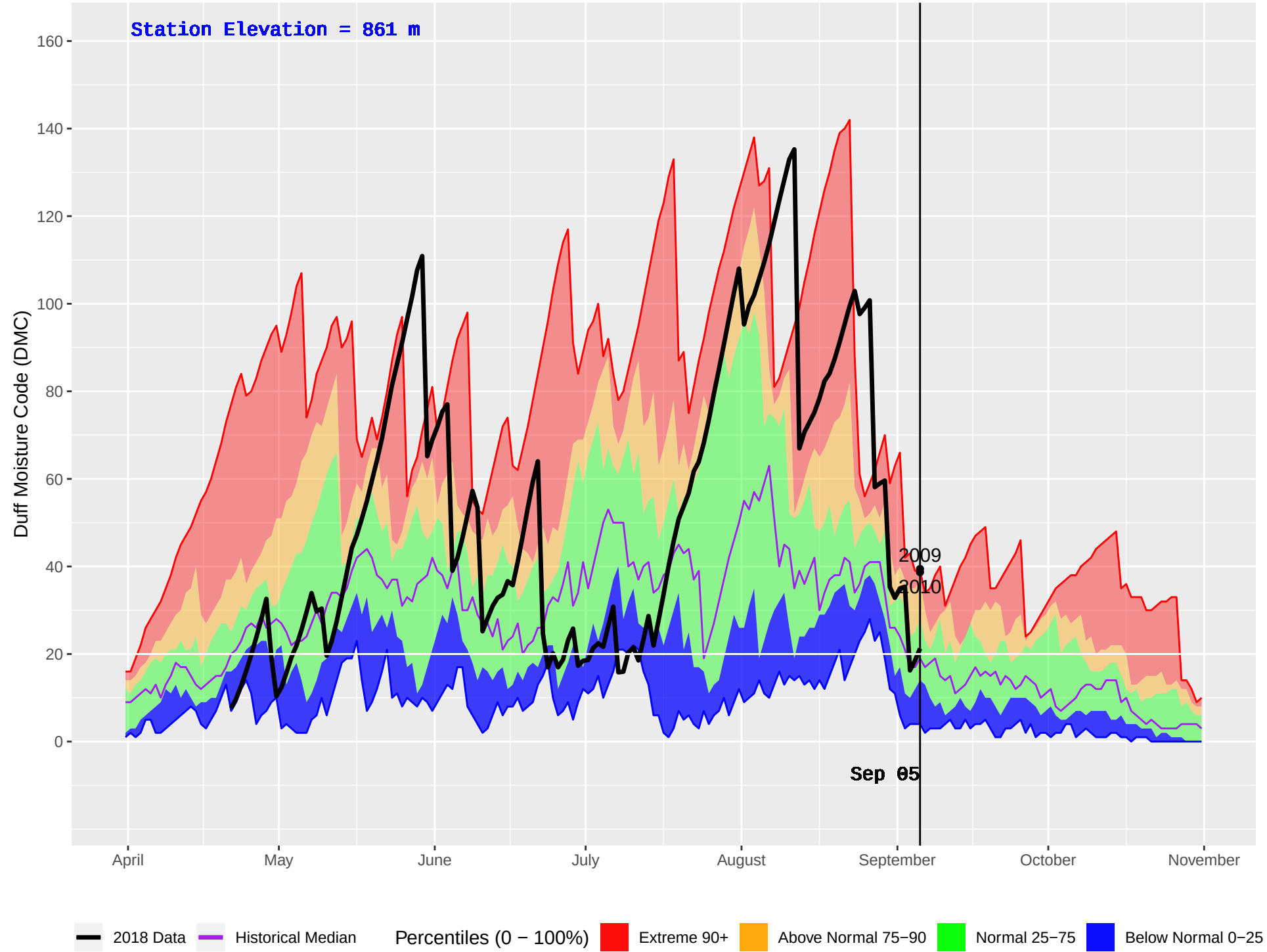
BLAEBERRY (866) : Historical (2004–2016) and Current (2018) Daily Duff Moisture Code (DMC)
