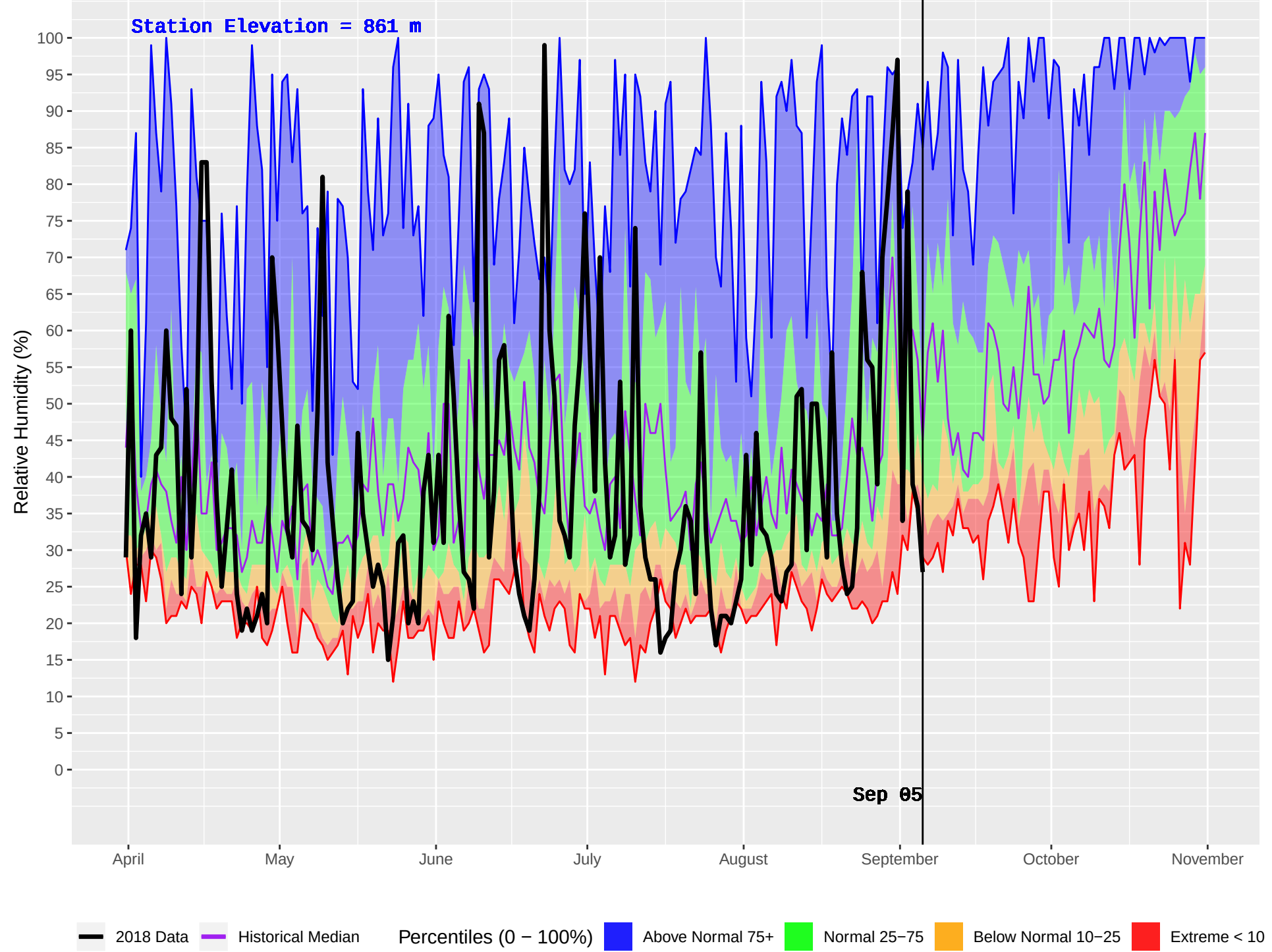
BLAEBERRY (866) : Historical (2004–2016) and Current (2018) Daily Relative Humidity
